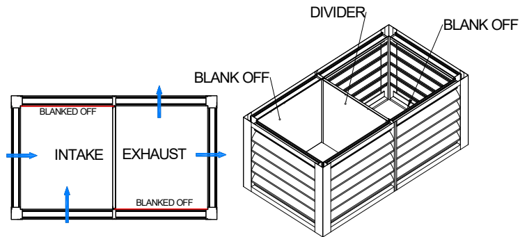
DIVIDER / BAFFLE
