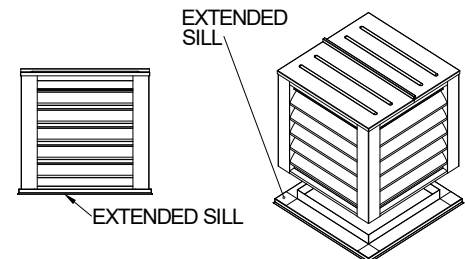
EXTENDED SILL / NO BOTTOM FLANGE
