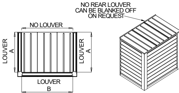
3 SIDED PENTHOUSE
